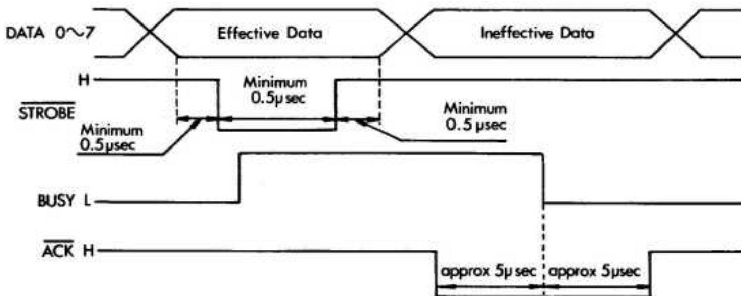
DATA input waveform
