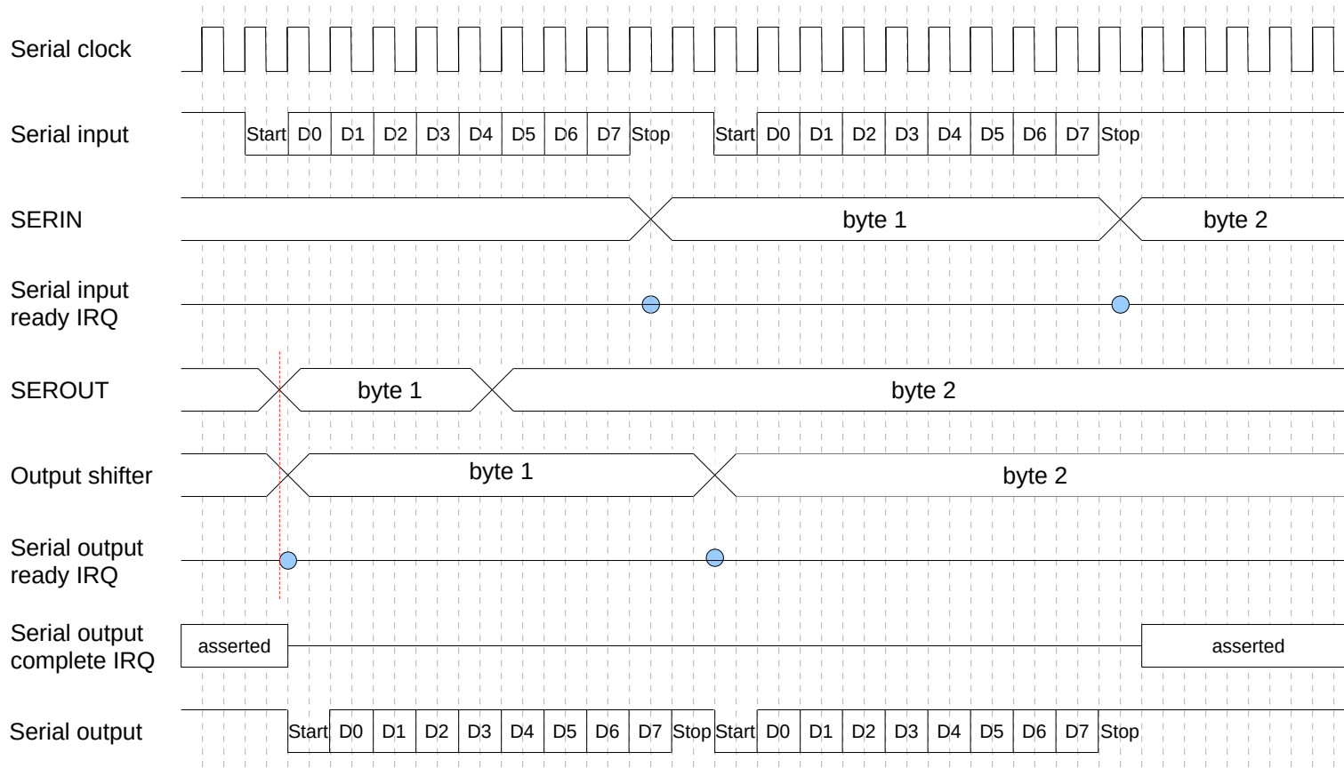
Figure 11: POKEY synchronous serial receive/transmit timing
