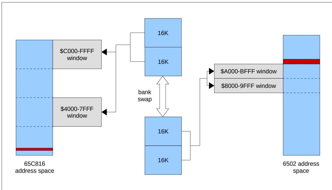
Figure 13: Veronica memory layout
