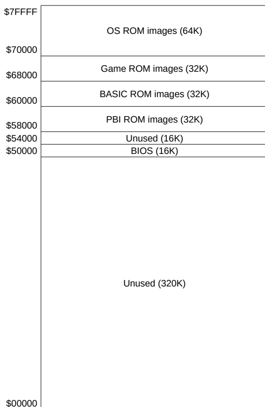
Figure 18: Ultimate1MB flash memory map
