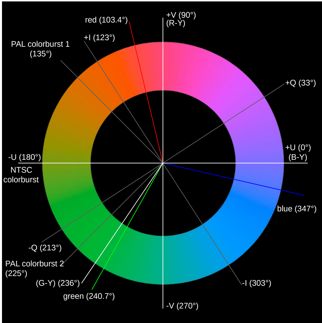
Figure 19: YIQ/YUV color space relations
