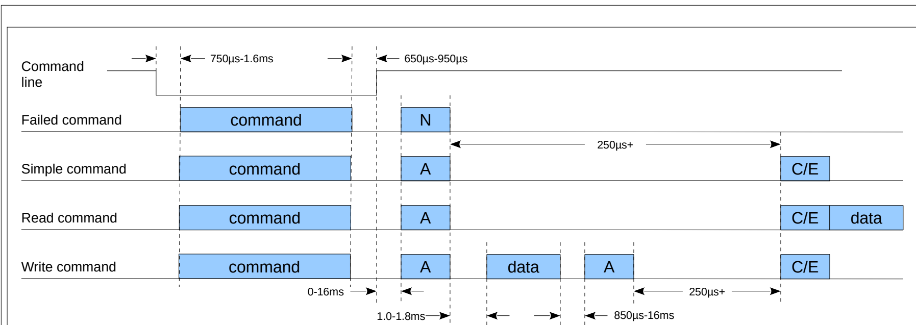
Figure 14: SIO command timing
