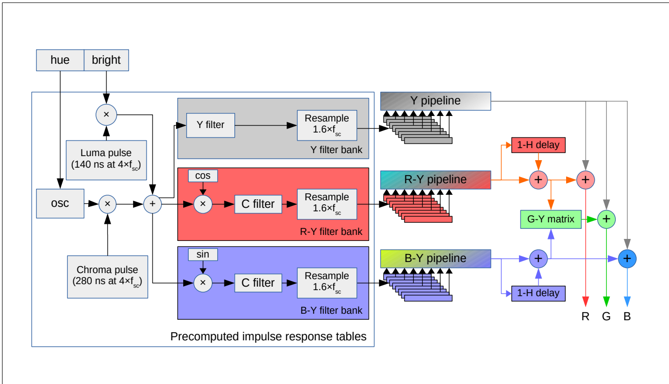
Figure 22: Altirra PAL high artifacting pipeline
