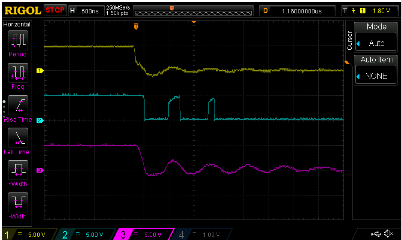
Figure 12: CX-75 triggering glitch on NTSC 800XL
