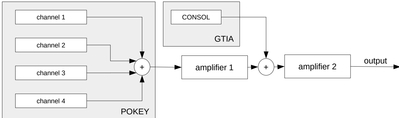
Figure 23: Analog audio block model
