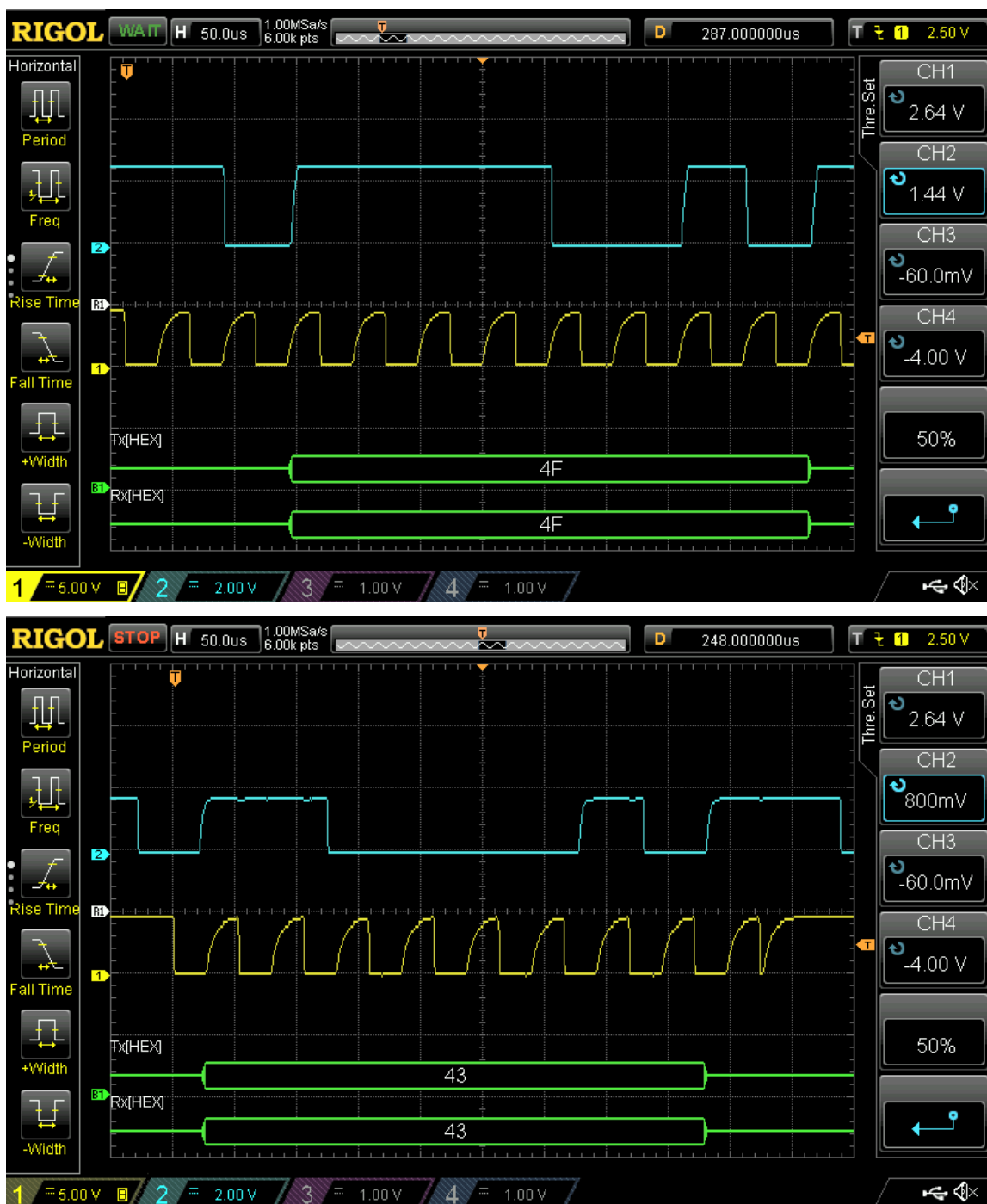
Figure 9: SIO send/receive clocking signals
