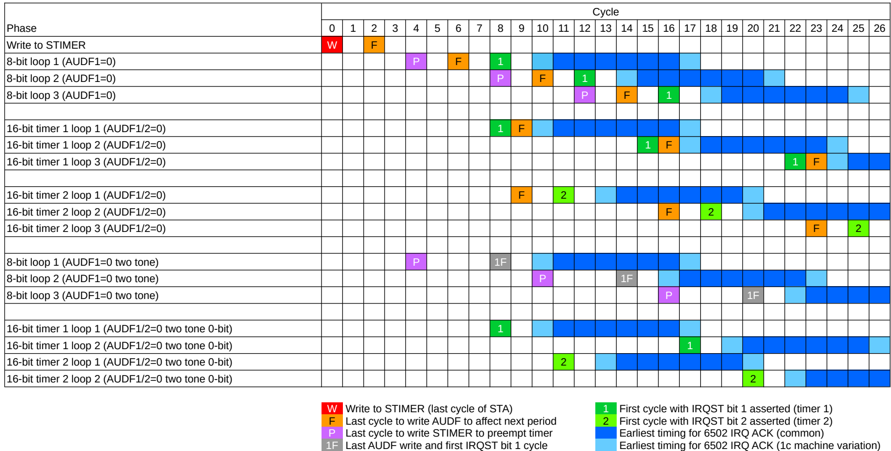
Figure 8: POKEY detailed timer timing
