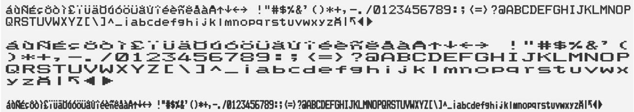
Figure 16: 1025 character set
