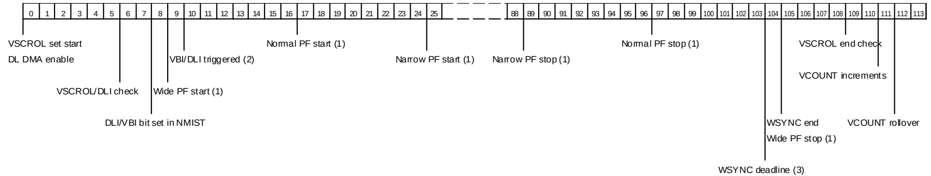
Figure 6: ANTIC event timing
