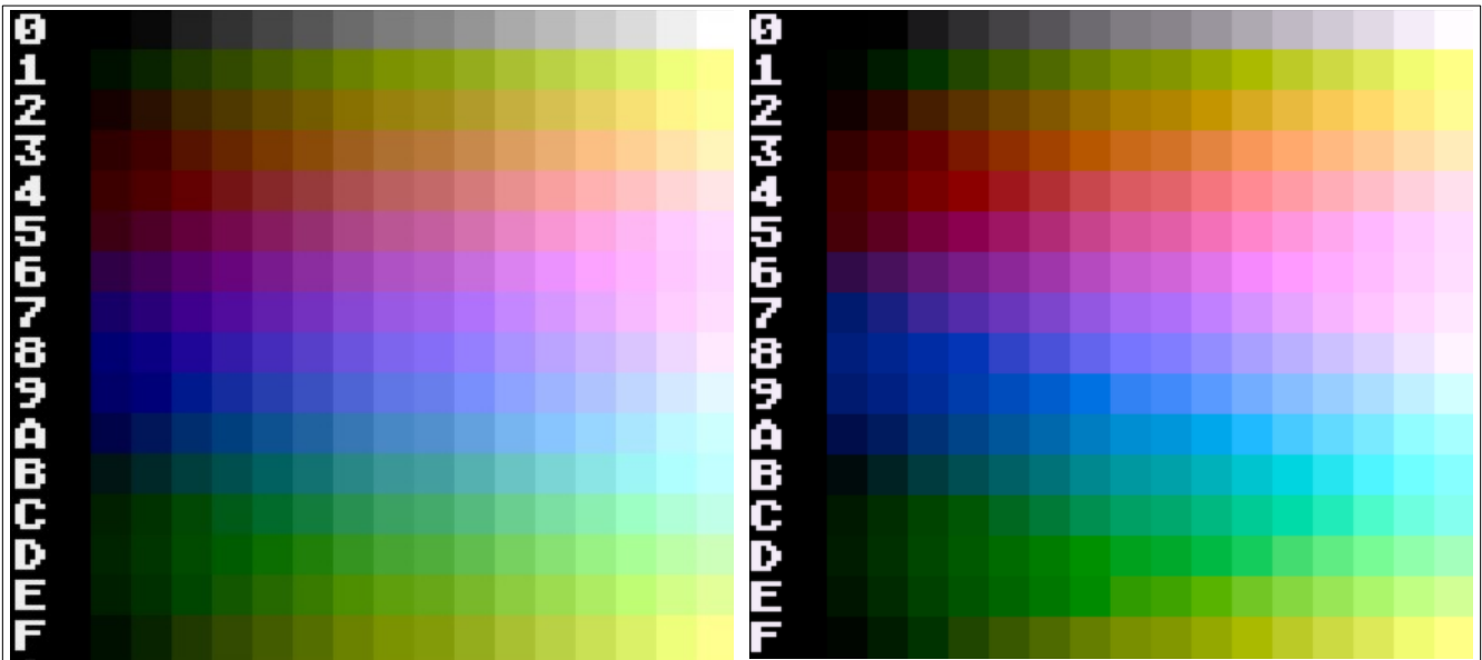
Figure 20: Effect of color correction on computed palette
