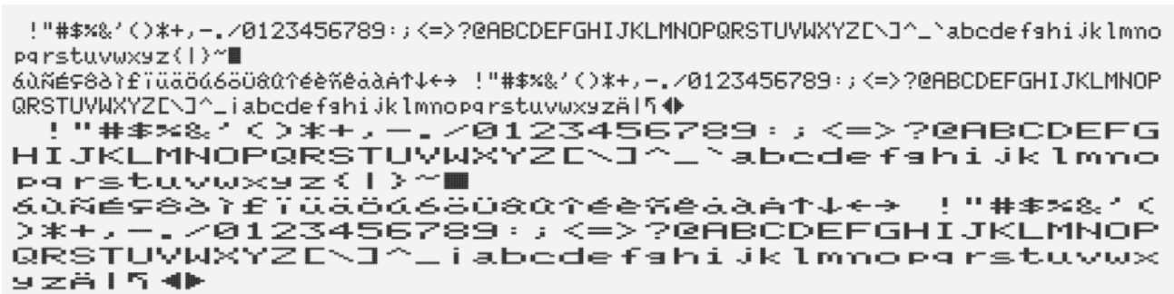
Figure 17: 1029 character set
